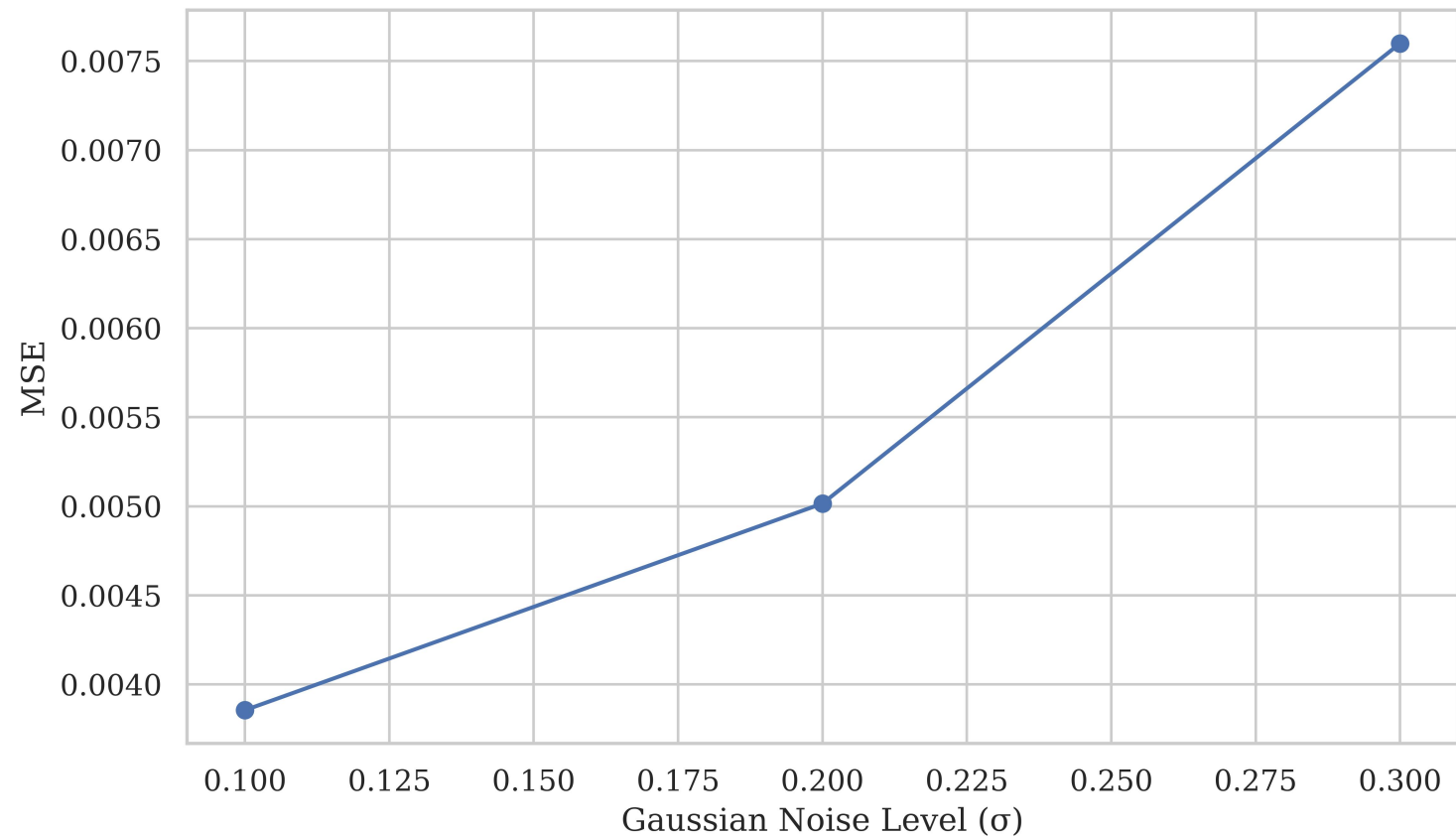
Noise Level vs MSE
